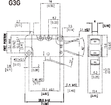
Dimensions G3G
