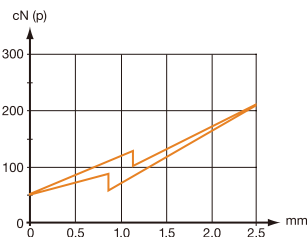
Actuating force/travel
